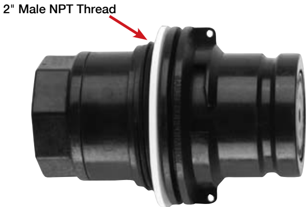
Male Adapter Dry Poppet DPCMT100
